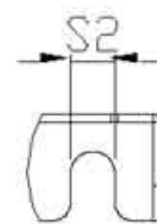
Detail B (Mounting Hole)
