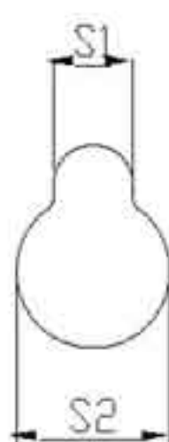
Detail A (Mounting Hole)
